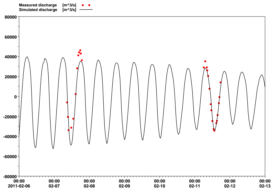
Figure 4.10 Discharge validation at Akram Point in Sibsa river during the dry season (February 2011)
