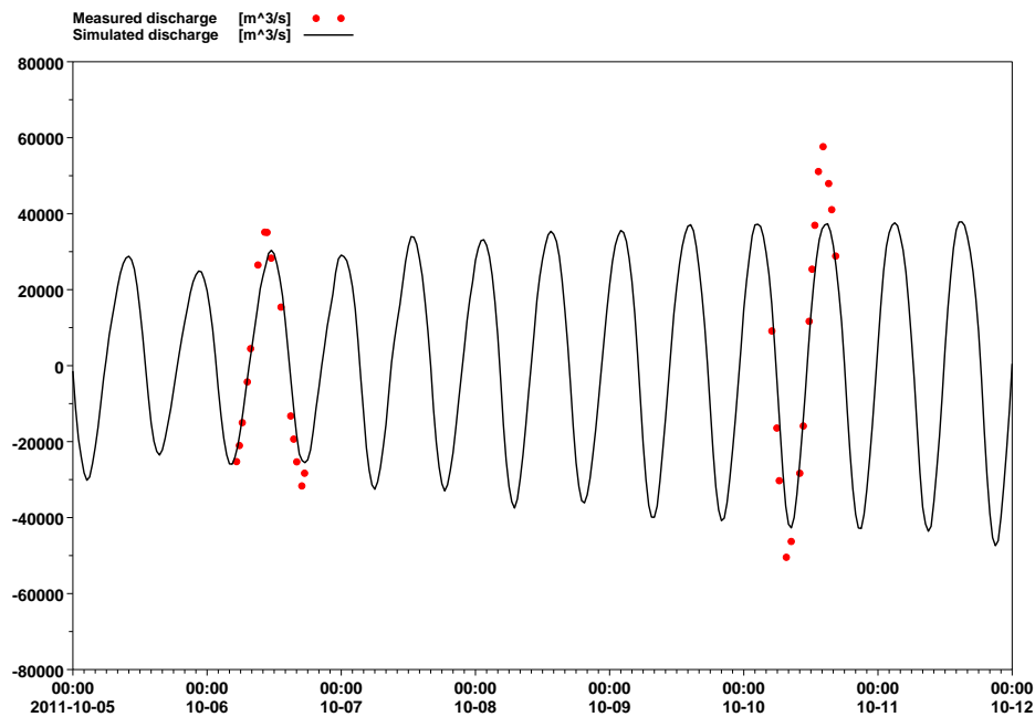
Figure 4.9 Discharge calibration at Akram Point in Sibsa river during monsoon (October 2011)
