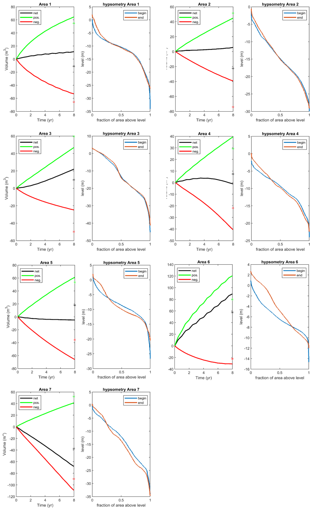
Figure 4.17 Cumulative modelled erosion volumes, deposition volumes and area-net volumes (left panels) and hypsometries at the start (2011) and end (2019) (right panels) for different areas as defined in Figure 4.16. Observed volumes are indicated by (*)
