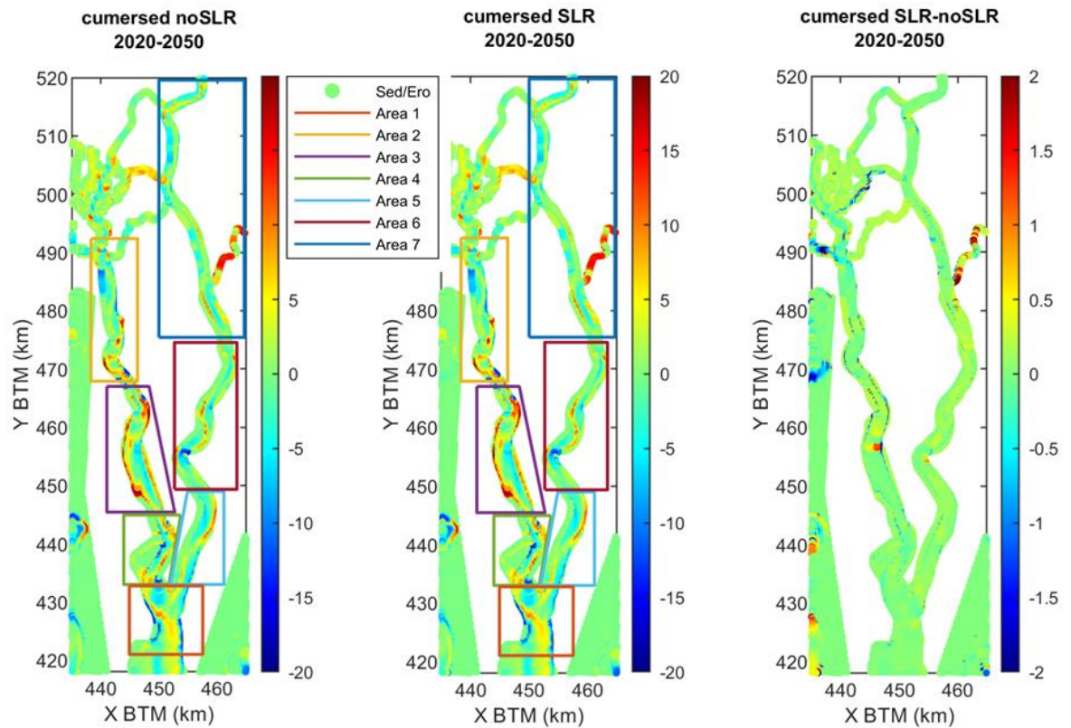
Figure 7 Sedimentation/erosion in Pussur-Sibsa system, 2020-2050. Left panel: no SLR, Mid panel: 1m SLR and Right Panel: The effect of 30 cm SLR on bed level change between 2020 and 2050. Negative values denote erosion by SLR.
