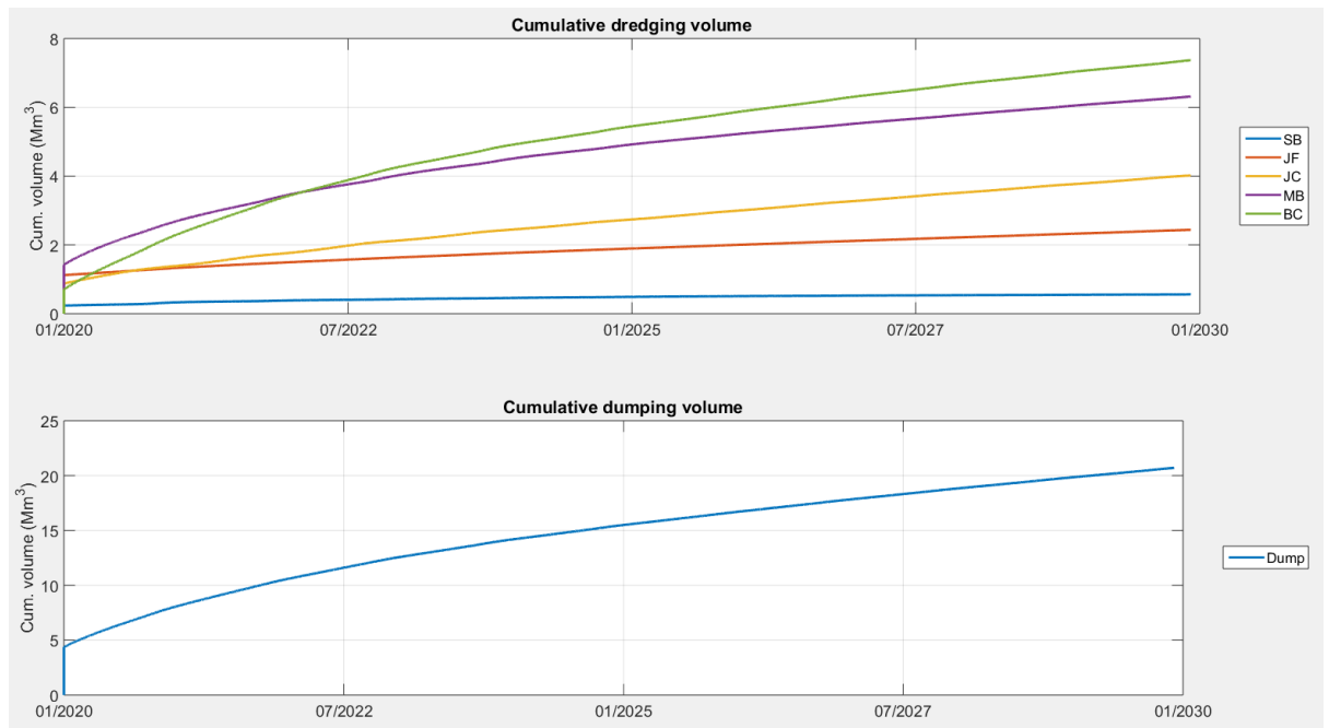
Figure 25 Dredging volume of individual area SB, JF, JC, MB & BC (upper panel) and Dumping of total dredging volume for all the areas
