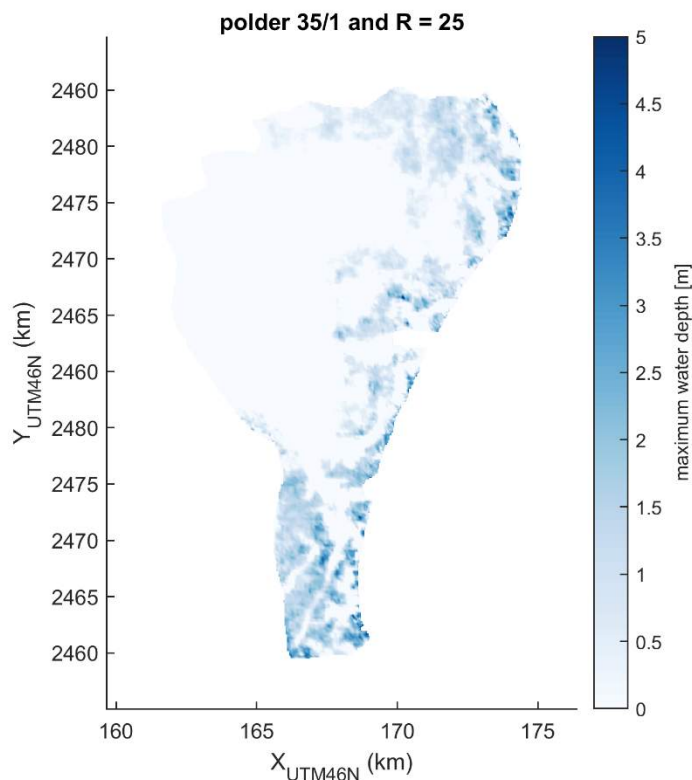
Figure 2-9 25-year return period for polder 35/1, including relative sea level rise
