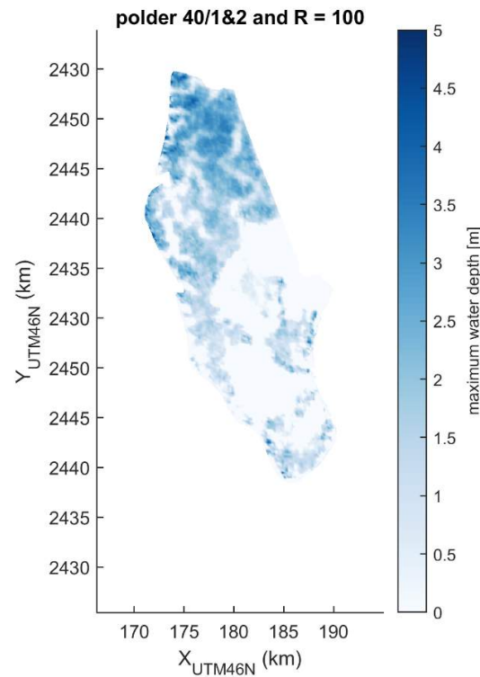
Figure 2-6 No relative SLR and R=100 years
