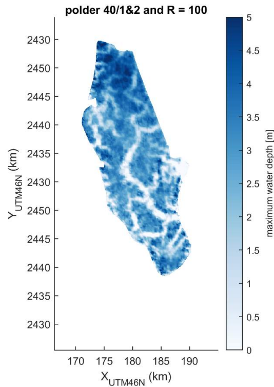
Figure 2-8 With relative SLR and R=100 years
